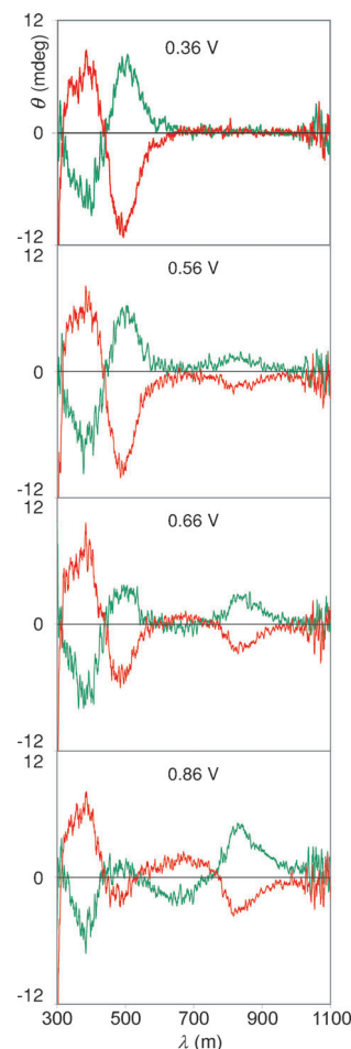
Figure 3. CD spectra of films of oligo-(R)-(-)- 1a (red) and oligo-(S)-(+)- 1a (green) on an ITO electrode during an anodic cycle in 0.1 M (TBA) \text{PF}_6 in acetonitrile. Potentials are referred to the \text{Fc}^+/\text{Fc} couple.
