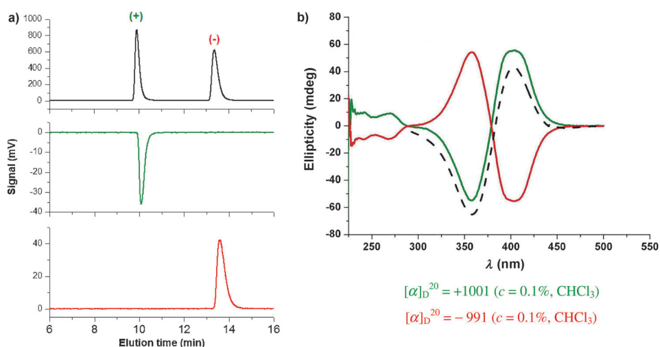
Figure 1. a) Analytical HPLC resolution of ( \pm )-1a and purity check of the enantiomers isolated on a semipreparative scale. Column: Chiralpak IB-3 (250 \times 4.6 mm I.D.); eluent: n -hexane/CH 2 Cl 2 /EtOH = 100:5:0.2 (v/v/v); T = 25^\circ\text{C} ; (detector UV at \lambda = 360 \text{ nm} , detector CD at \lambda = 360 \text{ nm} ). Black: ( \pm )-1a; green: first eluted enantiomer, (+)-1a; red: second eluted enantiomer, (-)-1a. b) CD spectra (CHCl 3 , c = 0.14 \text{ mg cm}^{-3} ) of (S)-(+)-1a (green) and (R)-(-)-1a (red). Dotted black curve: calculated CD spectrum for (S)-1a.
